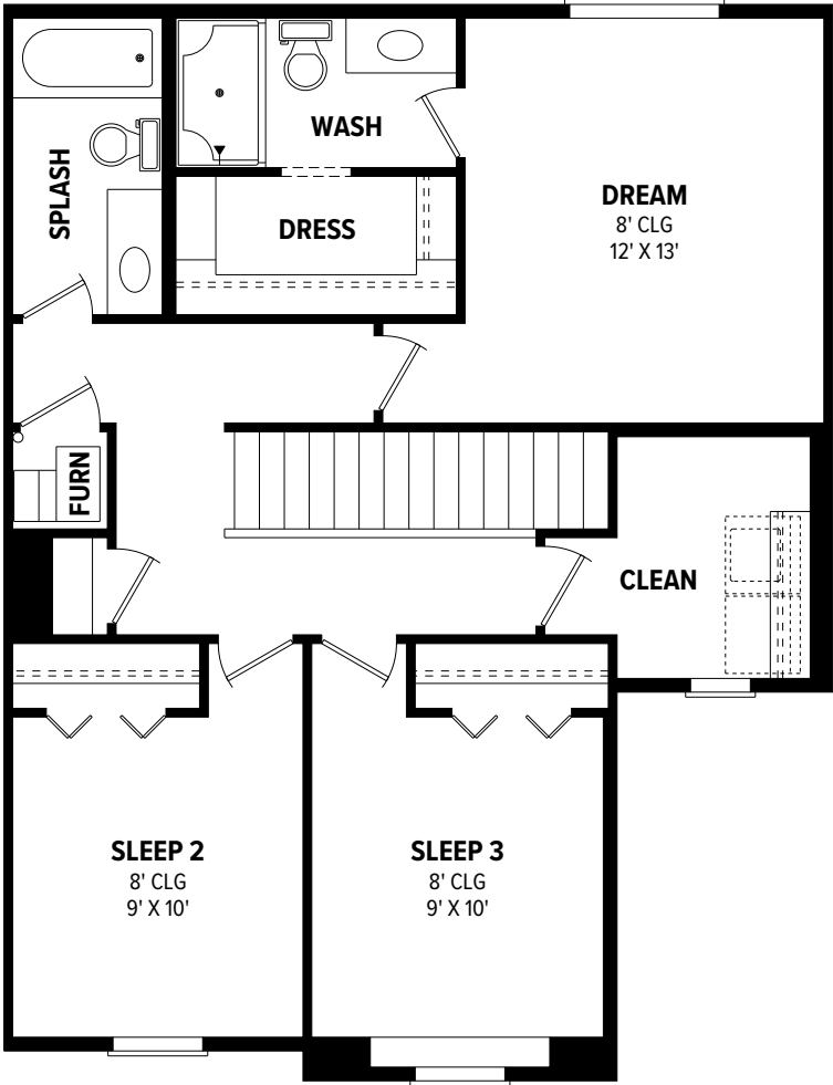
UPPER LEVEL
