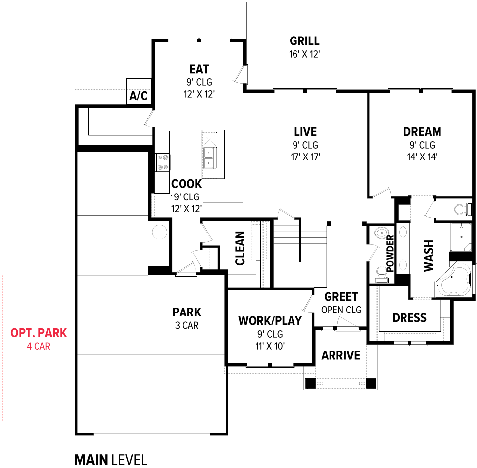
FLOOR PLANS
