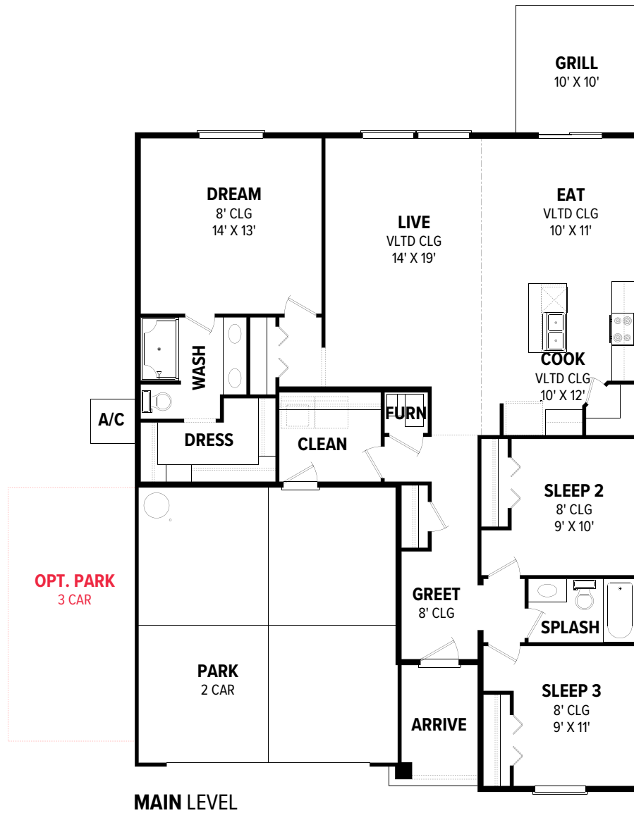
FLOOR PLAN
