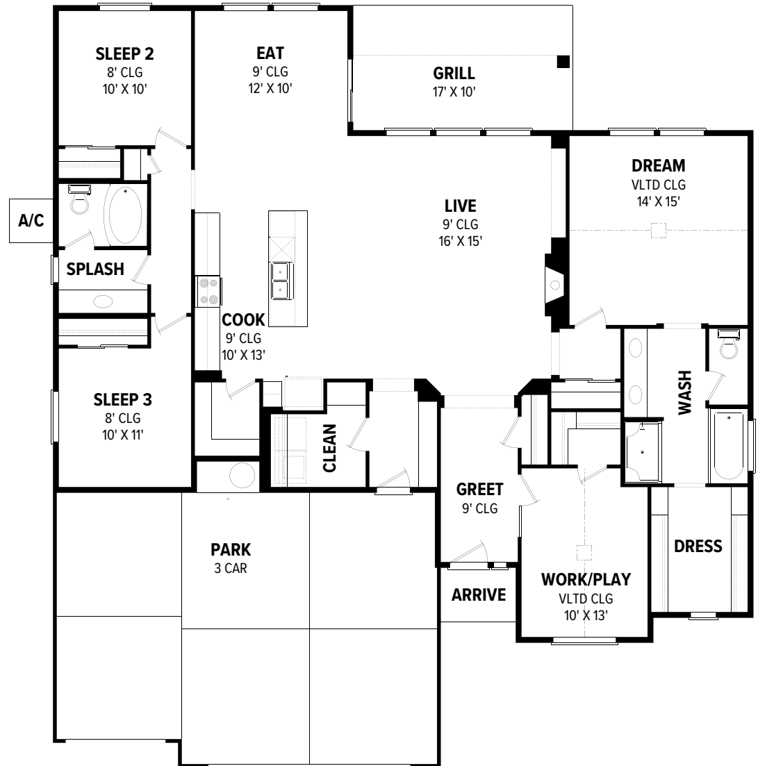
MAIN LEVEL
