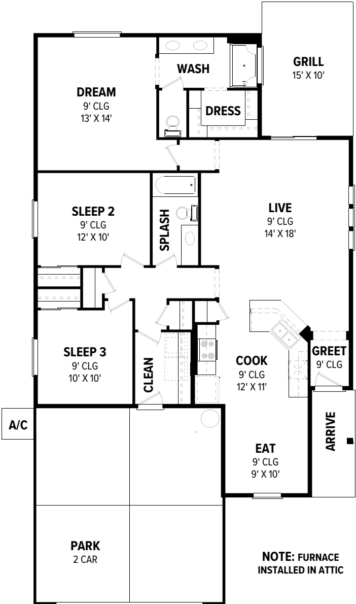
MAIN LEVEL
