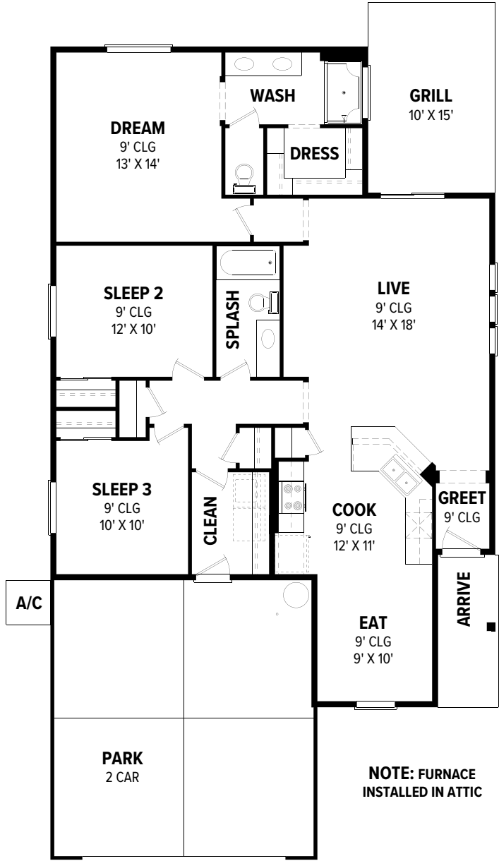
MAIN LEVEL
