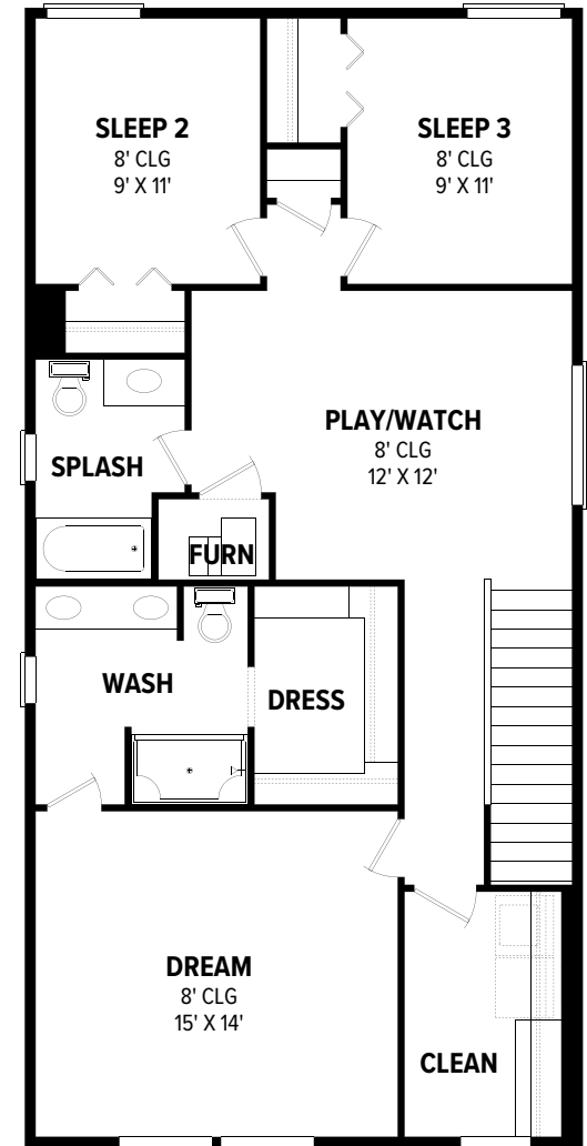
UPPER LEVEL
