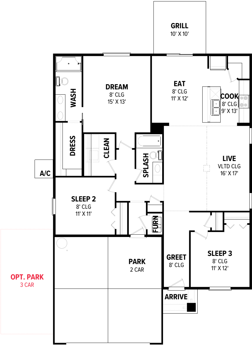
MAIN LEVEL
