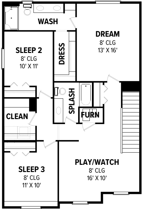
UPPER LEVEL
