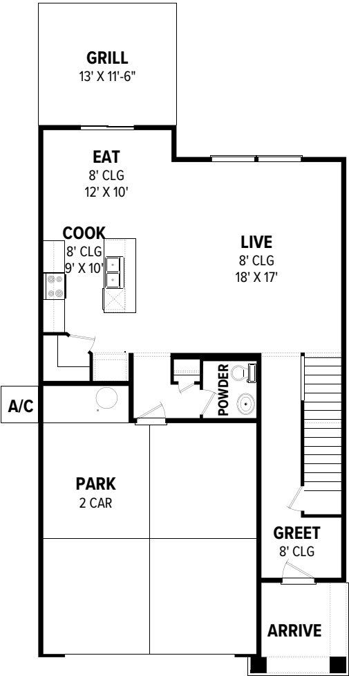
MAIN LEVEL
