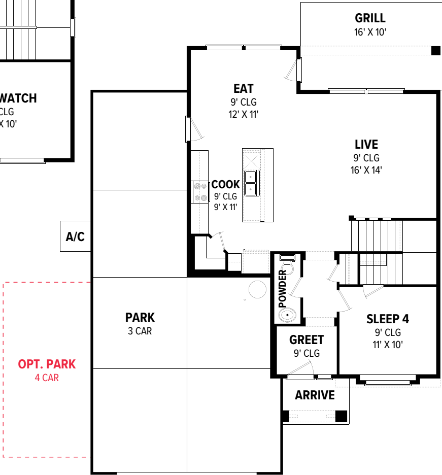
MAIN LEVEL
