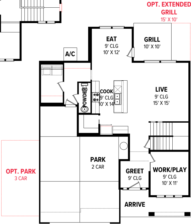
MAIN LEVEL
