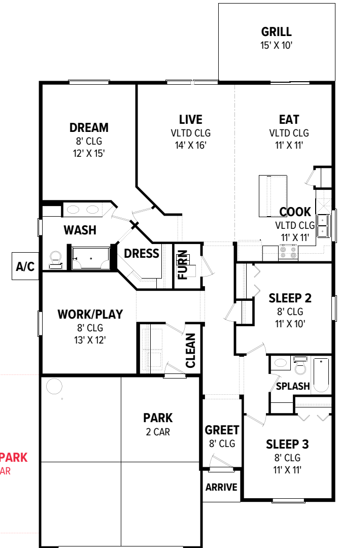
MAIN LEVEL
