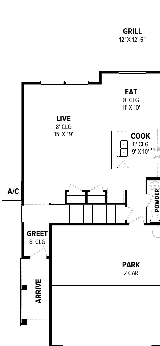
MAIN LEVEL
