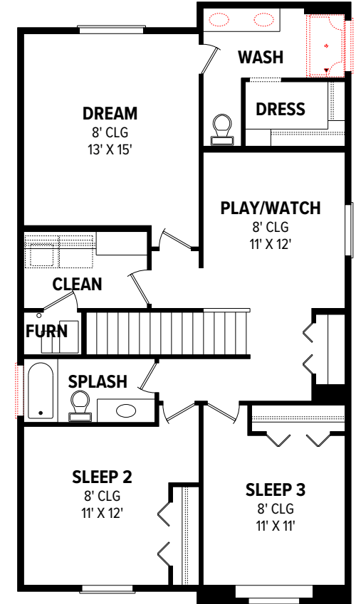
UPPER LEVEL
