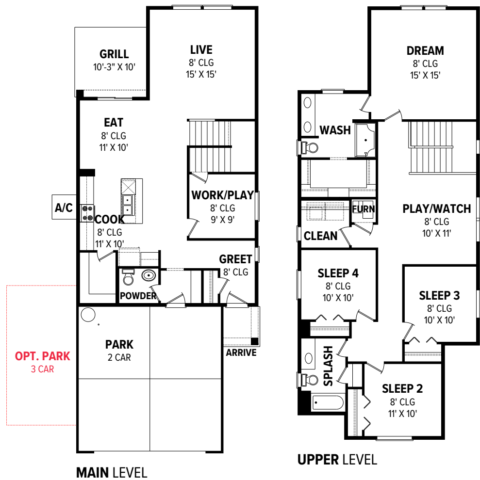
FLOOR PLANS
