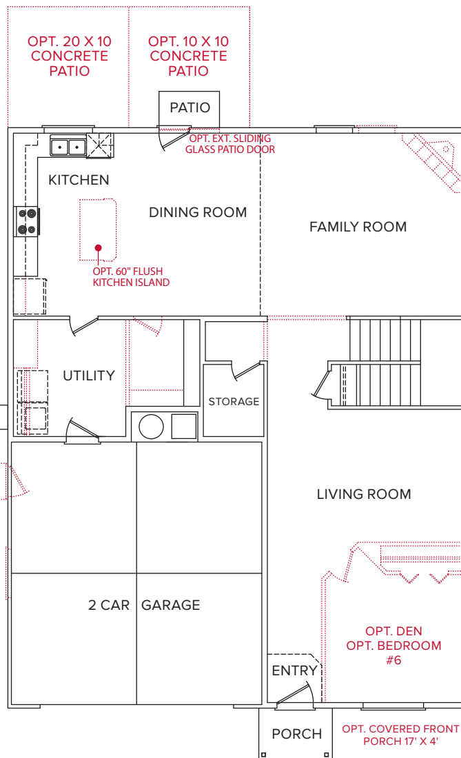
MAIN LEVEL
