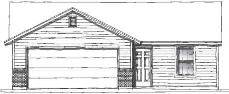
:: CLASSIC ELEVATION ::
