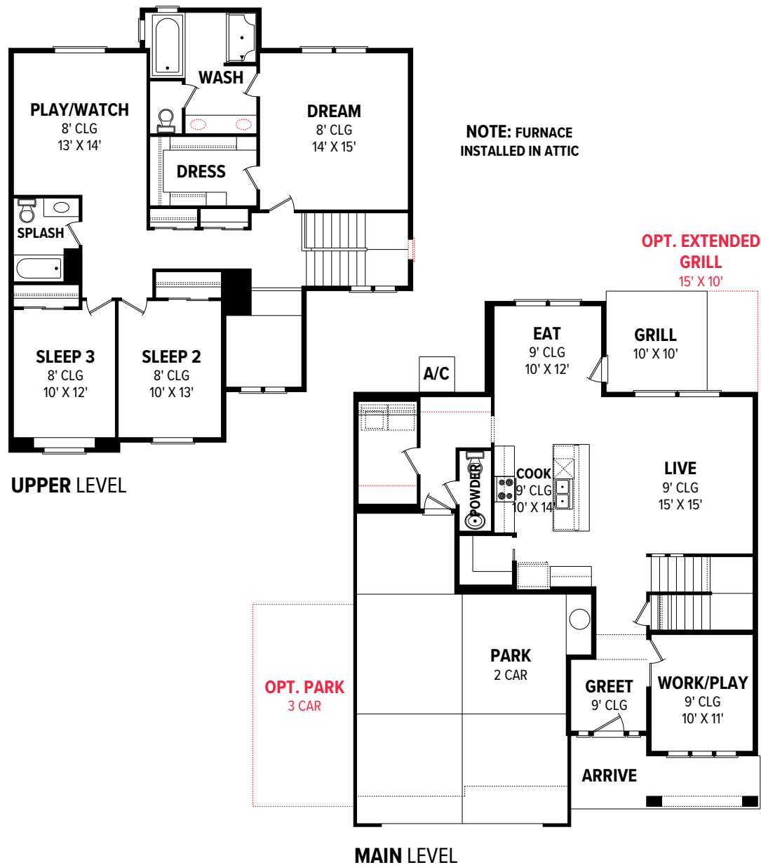
FLOOR PLANS
