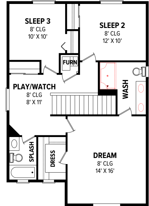
UPPER LEVEL
